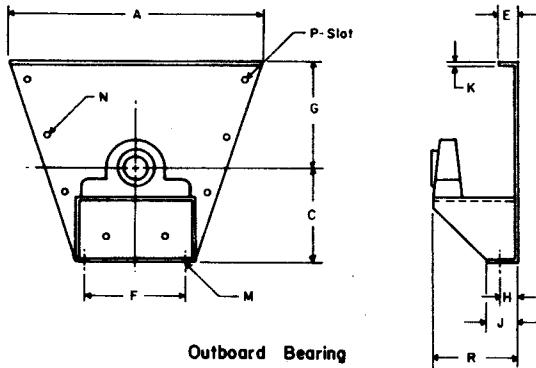
Outboard Bearing
